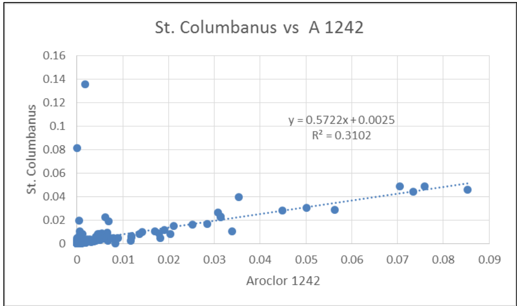
Figure 3-26: Comparison of mass fractions for gas-phase PCBs at St. Columbanus and Aroclor 1242
